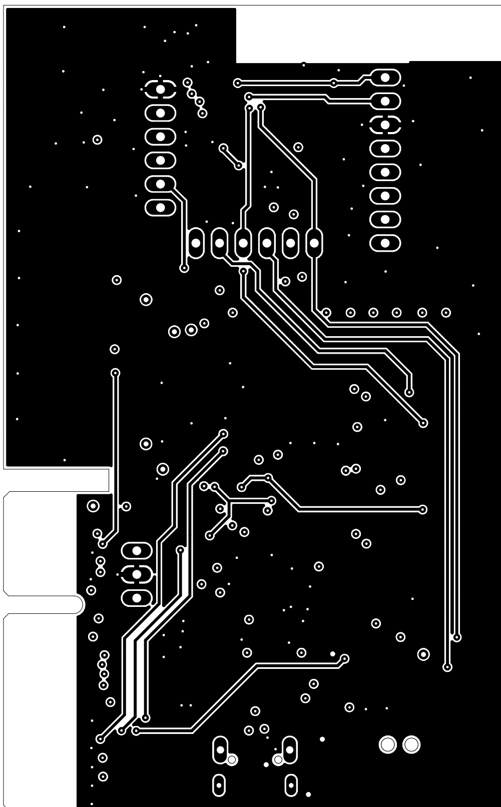
Figure 16: Bottom
