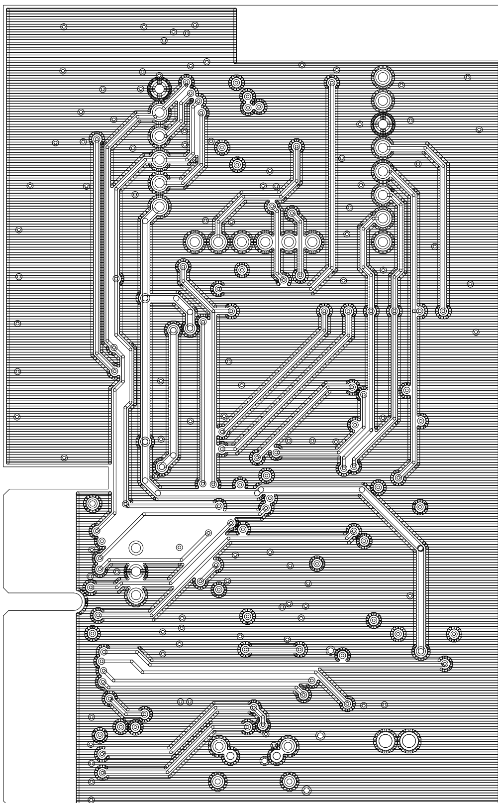
Figure 15: Layer 3
