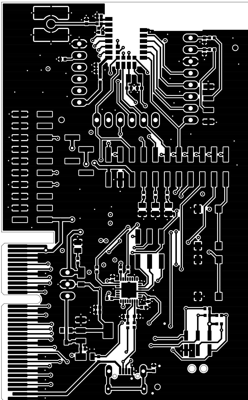
Figure 13: Top
