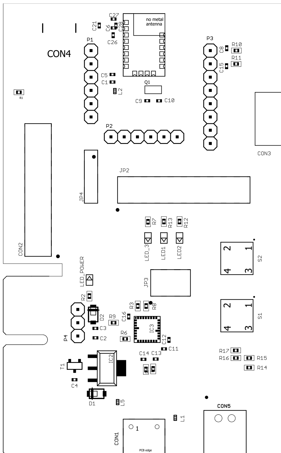
Figure 12: Assembly diagram
