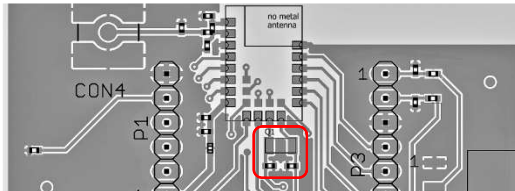
Figure 9: LFXO mounting
